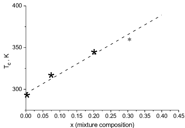
Fig. 3. The dependence of T_C for \text{SbO}_x\text{S}_{1-x}\text{I} upon the mixture composition.
