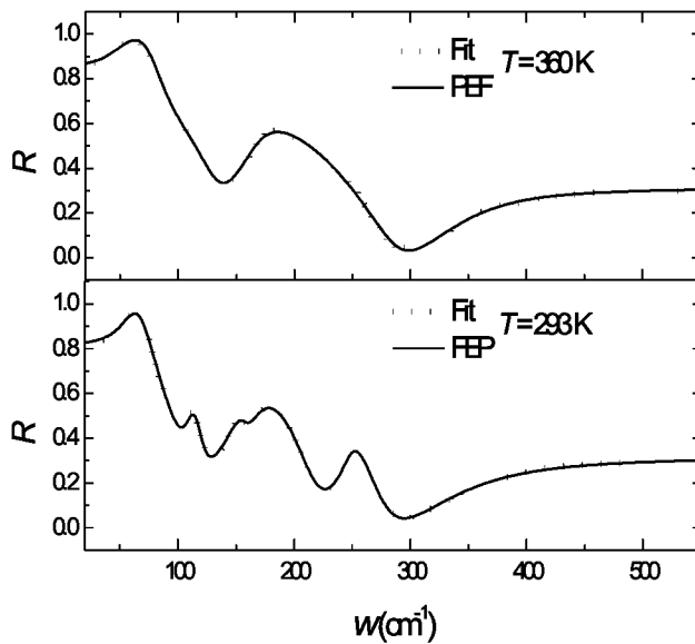
Fig. 4. The reflection spectrum R(\omega) of the \text{SbO}_x\text{S}_{1-x}\text{I} ( x = 0.2 ) crystals studied by the OP technique at \mathbf{E} \parallel \mathbf{c} and T = 293 K (FEP), T = 360 K (PEP).
