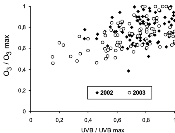
Fig. 5. Scatter plot of normalized UVB radiation intensity and the ground-level ozone concentrations in April–June.
