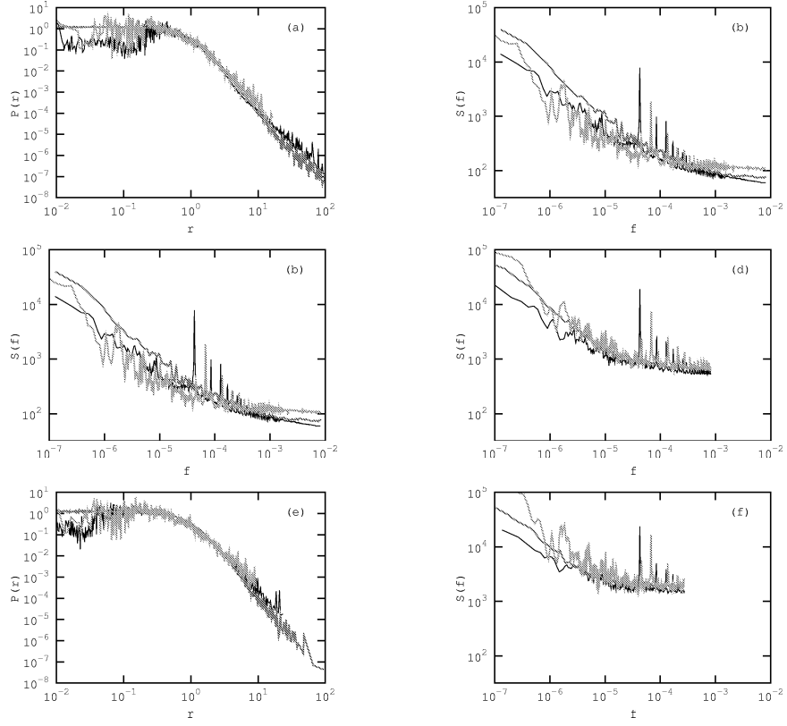
Figure 1: Comparison of empirical statistics of absolute returns traded on the NYSE (black thin lines) and VSE (light gray lines) with model statistics, (1)-(7), (gray lines). Model parameters are as follows: \lambda = 5 ; \sigma_t^2 = 1/3 \cdot 10^{-6} s^{-1} ; \lambda_0 = 3.6 ; \epsilon = 0.017 ; \eta = 2.5 ; \bar{r}_0 = 0.4 ; x_{max} = 1000 . PDF of normalized absolute returns is given on (a), (c), (e) and PSD on (b), (d), (f). (a) and (b) represents time series with \tau = 60s ; (c) and (d) \tau = 600s ; (e) and (f) \tau = 1800s . Empirical data from NYSE is averaged over 24 stocks, empirical data from VSE is averaged over 4 stocks and model data is averaged over 100 realizations.
