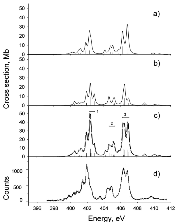
Fig. 1. Sc 2p photoabsorption spectrum. Calculation in CI approximation (1): (a) excitation from the {}^2D_{3/2} level, (b) excitation from {}^2D_{5/2} level, (c) excitation from the both levels of the ground term (thin line is CI approximation (1), thin broken line is single-configuration approximation, solid line at the higher end of the spectrum is photoionization), (d) experiment [1]. Vertical bars are intensities of lines in CI approximation (1), they have been convoluted using the average natural width. Numbers indicate the intervals of levels used for the excitation of emission spectrum.
