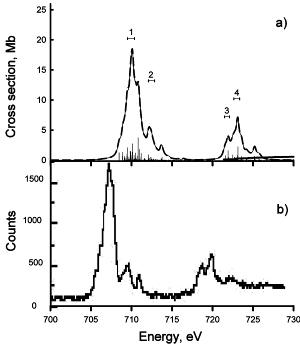
Fig. 3. Fe 2p photoabsorption spectrum: (a) calculation (thin line is CI approximation, thin broken line is single-configuration approximation, solid line is photoionization), (b) experiment [2]. Vertical bars are intensities of lines in CI approximation, they have been convoluted using the average natural width. Numbers indicate the intervals of levels used for the excitation of emission spectrum.
