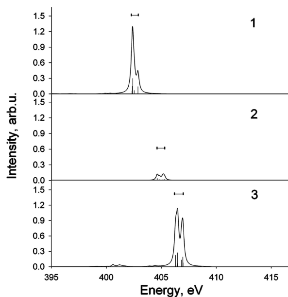
Fig. 2. Sc L_{2,3} emission spectrum generated at the photoexcitation to the groups of levels indicated in Fig. 1: 1 for 402.3–402.9 eV, 2 for 404.6–405.3 eV, 3 for 406.2–407.0 eV. Calculation in CI approximation, lines have been convoluted using the average natural width.
